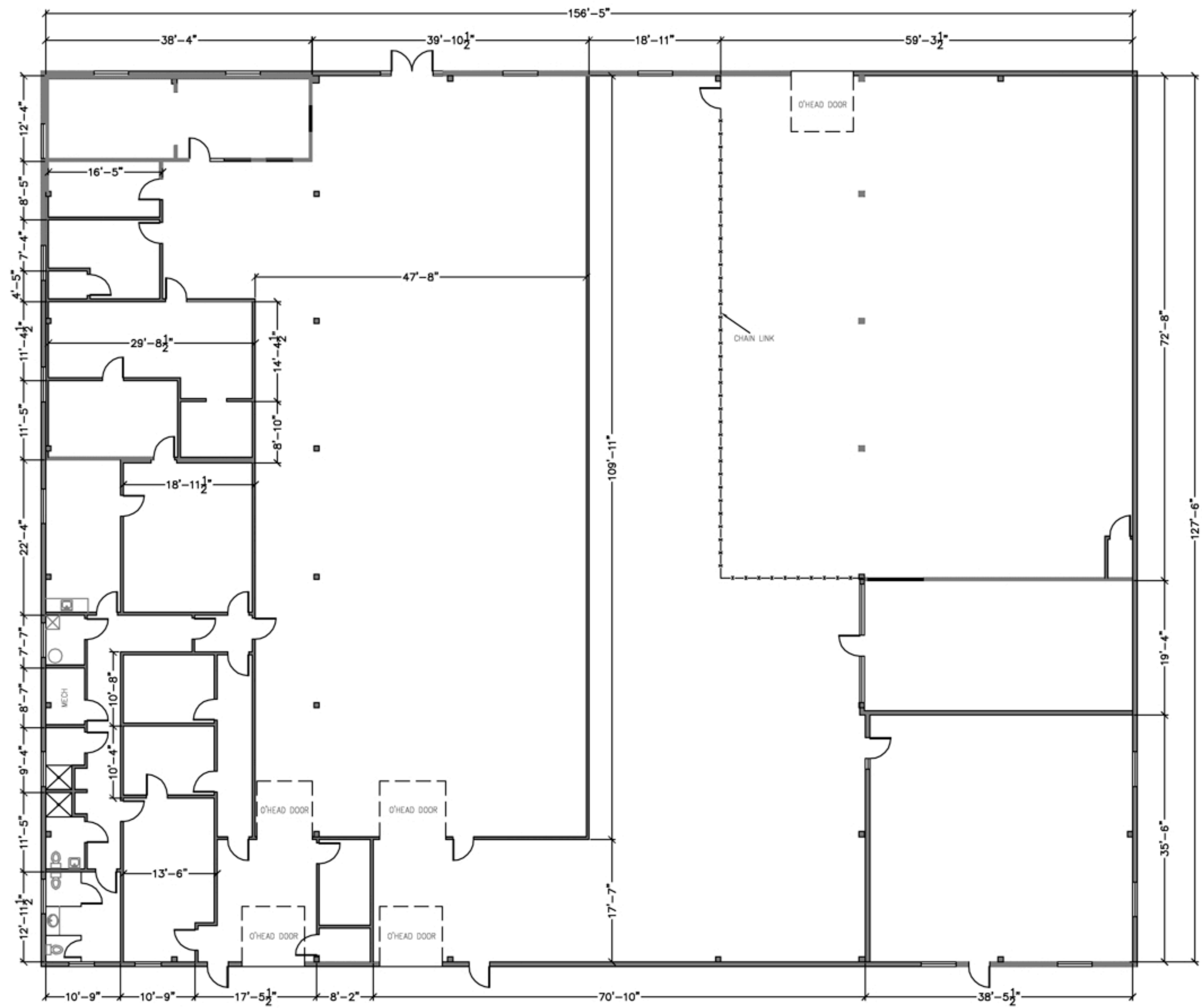
2000 E. 6TH ST. FLOOR PLAN
